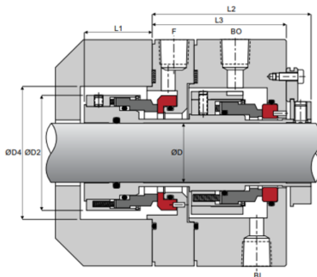
Optional Medium Pressure Design
