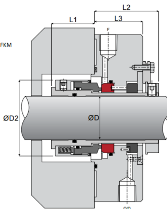
Optional Medium Pressure Design
